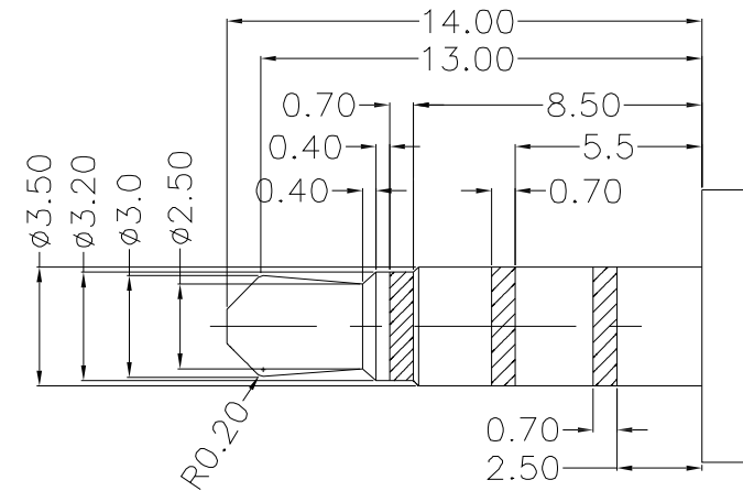
ø3.5mm 4POLE PLUG(TOLERANCE: ±0.05)
