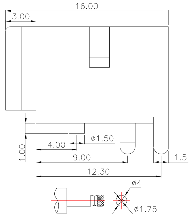
DC MATE PLUG
