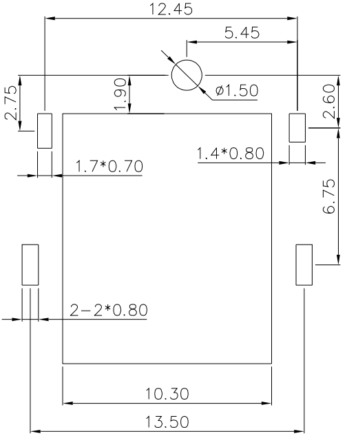
PCB LAYOUT
