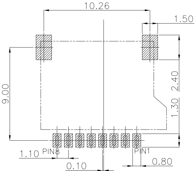
STEP III PUSH SHELL (C1/C2 SMITCH LOCK)
