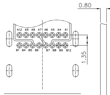
PCB BOTTOM SURFACE
